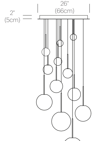
BOLA SPHERE CHANDELIER 4, 5, 6, 8, 10, 12 (X2)
