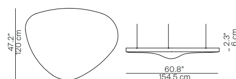
Lamp D71/2 (on/off) D71/2D (DALI) for D71P-D71C-D71P1
