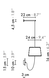
Tige murale / Fixed rod
