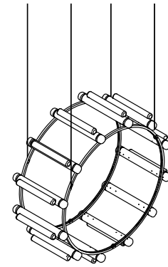
HORIZONTAL ORIENTATION
