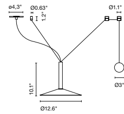
Milana 32 Counterweight
