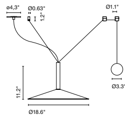
Milana 47 Counterweight
